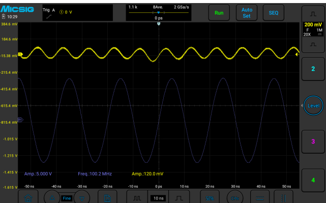
DP700, @100MHz, 5V, output common mode signal amplitude 120mV, CMRR is 32dB
