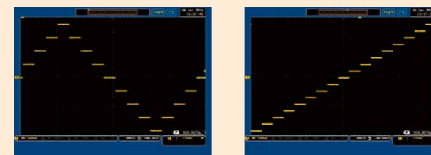
Staircase waveform
