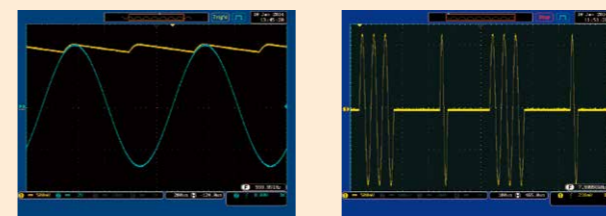
Full-wave rectifier circuit ripple waveform
